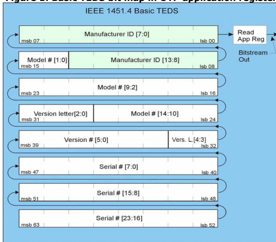
Figure 1: Basic TEDS bit map in OTP application register
